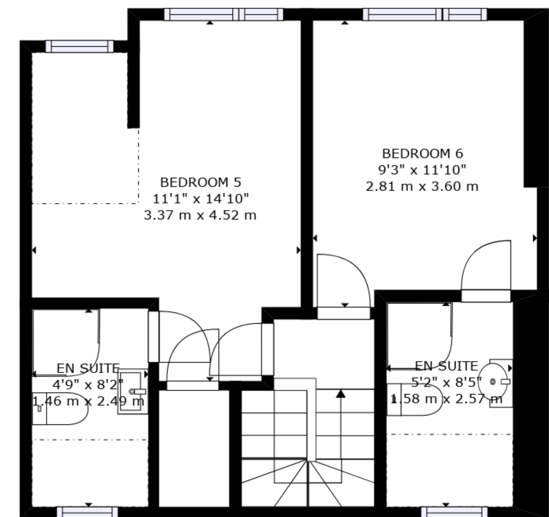
FLOOR 3
