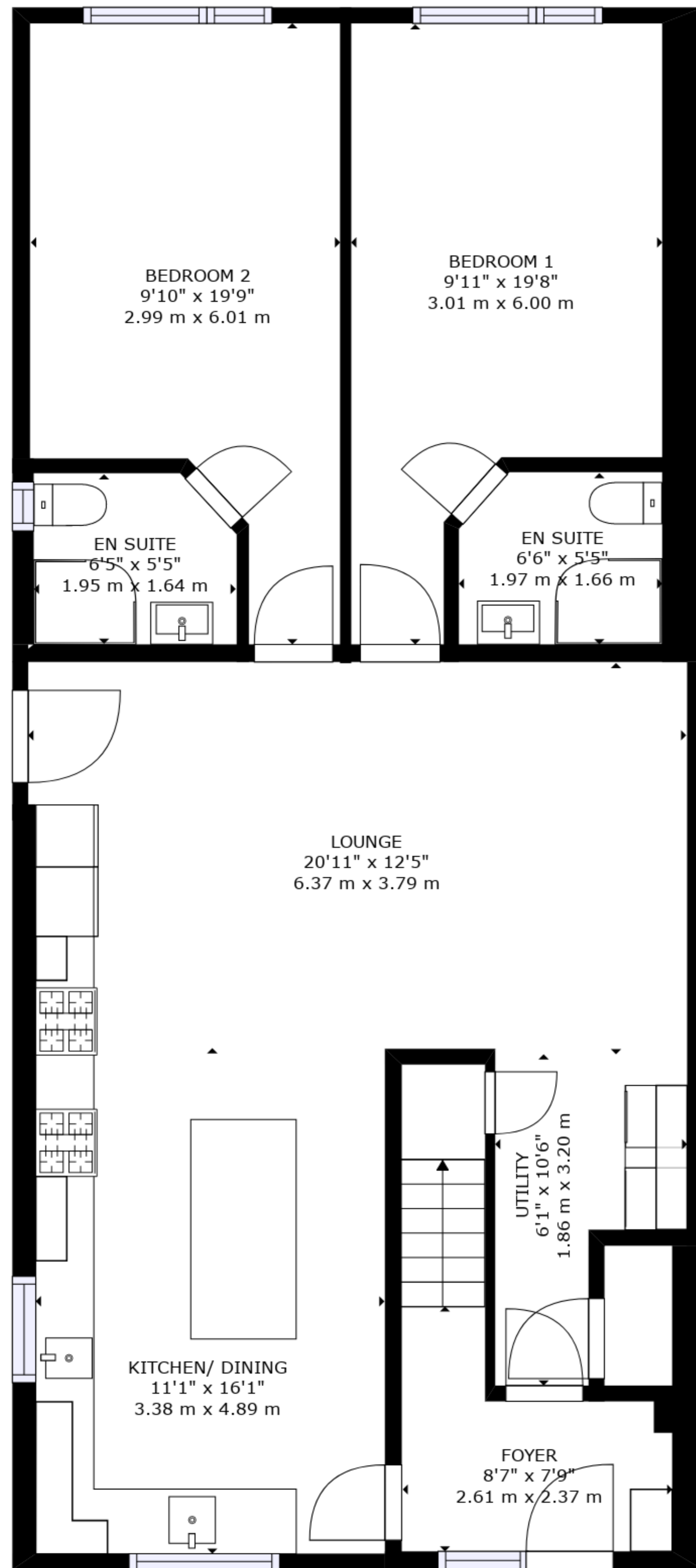
FLOOR 1
